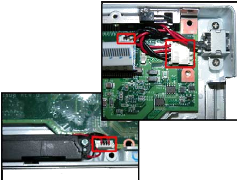
Fig. 31 Connectors on Main Board
